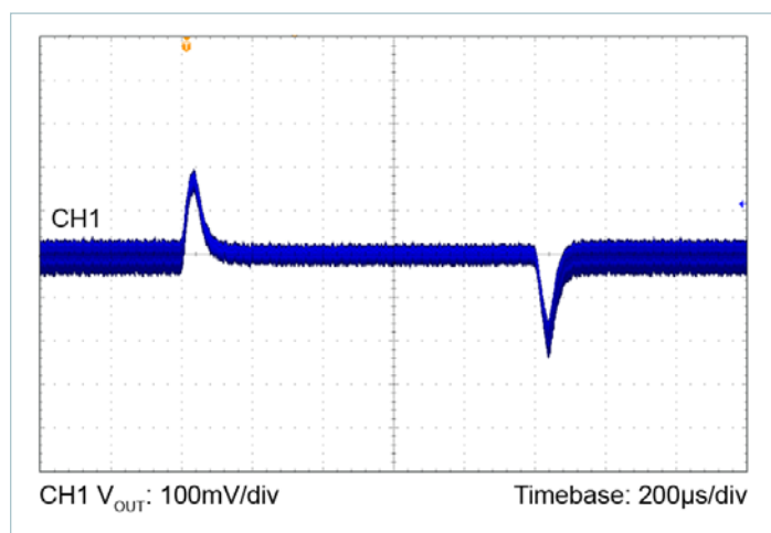
Figure 24 — 24V_{IN} to 10V_{OUT} , C_{OUT} = 8 \times 10\mu\text{F} ceramic 3.5 – 7.0A load step, 0.1A/ \mu s
