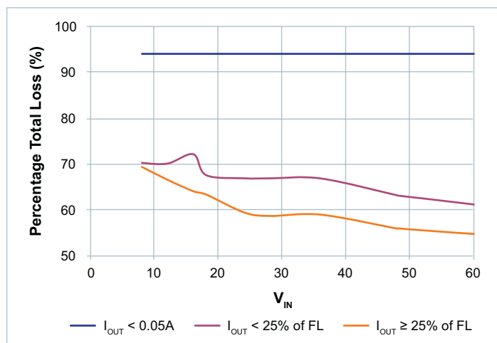
Figure 49 — V_{OUT} = 36V
