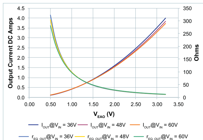
Figure 98 — r_{EQ\_OUT} vs. output current vs. V_{EAO} , V_{OUT} = 36V ; 36 – 60 V_{IN}
