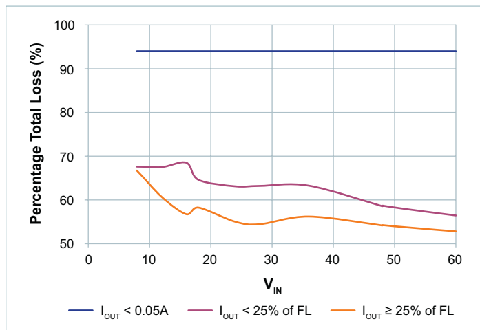
Figure 50 — V_{OUT} = 50V
