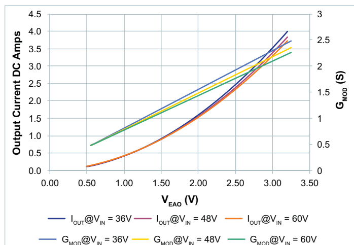
Figure 95 — G_{MOD} vs output current vs. V_{EAO} , V_{OUT} = 36V ; 36 – 60 V_{IN}
