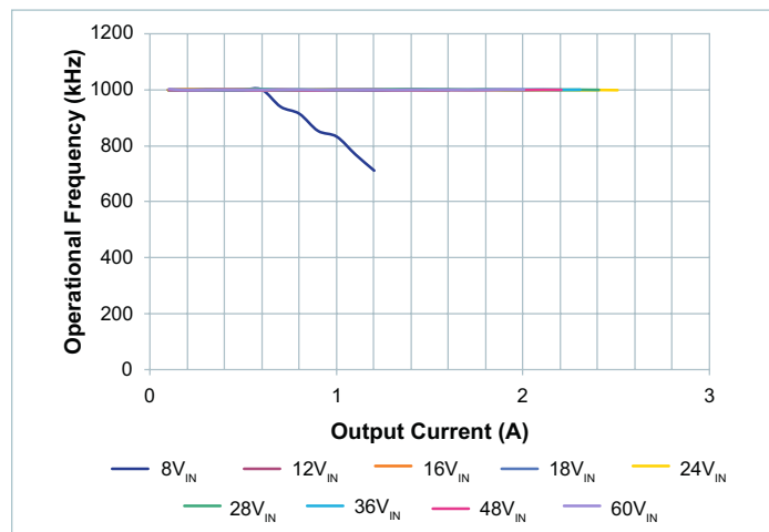
Figure 16 — Switching frequency vs. output current at 50V OUT
