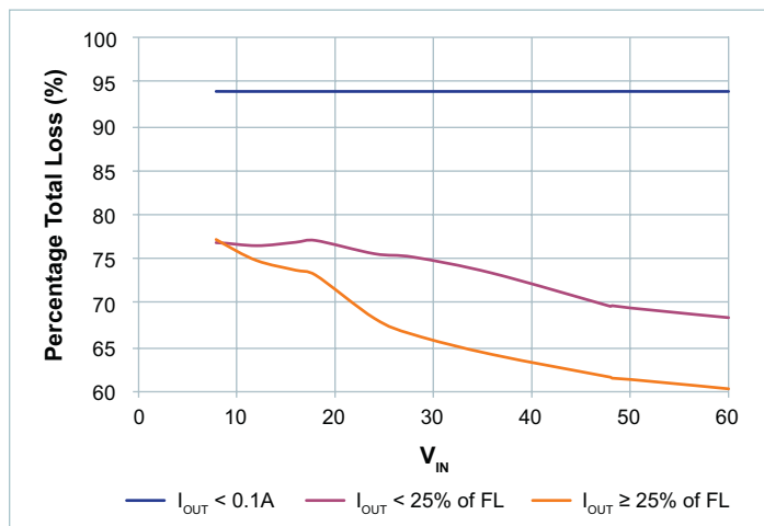
Figure 46 — V_{OUT} = 18V
