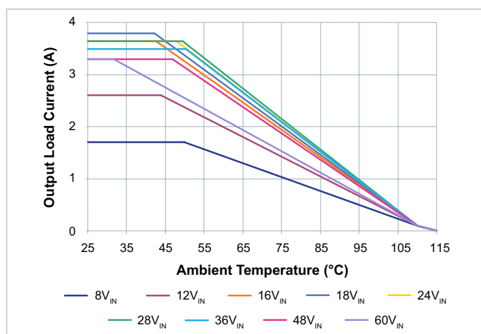
Figure 56 — Thermal de-rating for PI3740-00 evaluation board at V_{OUT} = 36V , 0LFM
