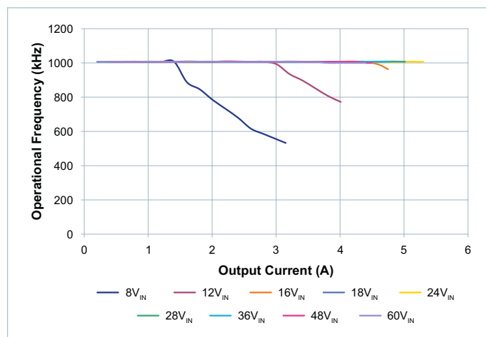
Figure 13 — Switching frequency vs. output current at 24V_{OUT}
