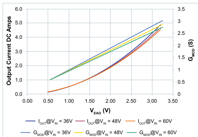
Figure 89 — G_{MOD} vs output current vs. V_{EAO} , V_{OUT} = 28\text{V} ; 36 – 60 V_{IN}
