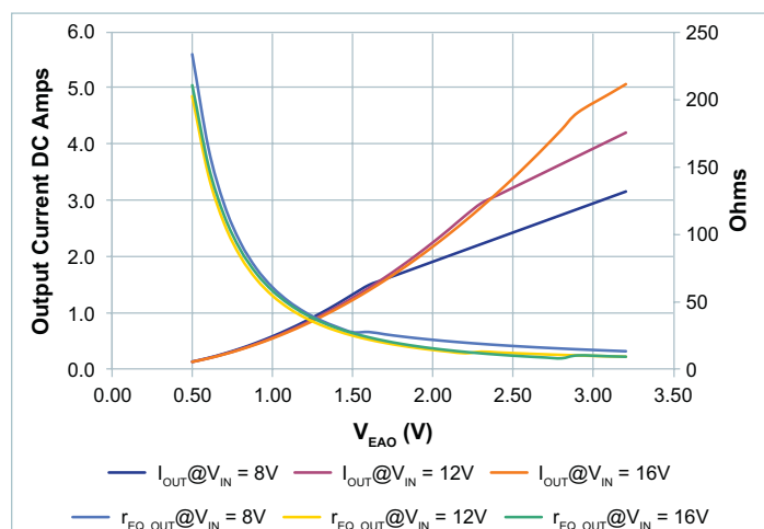
Figure 90 — r_{EQ\_OUT} vs. output current vs. V_{EAO} , V_{OUT} = 28\text{V} ; 8 – 16 V_{IN}
