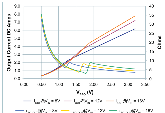
Figure 66 — r_{EQ\_OUT} vs. output current vs. V_{EAO} , V_{OUT} = 10V ; 8 – 16 V_{IN}
