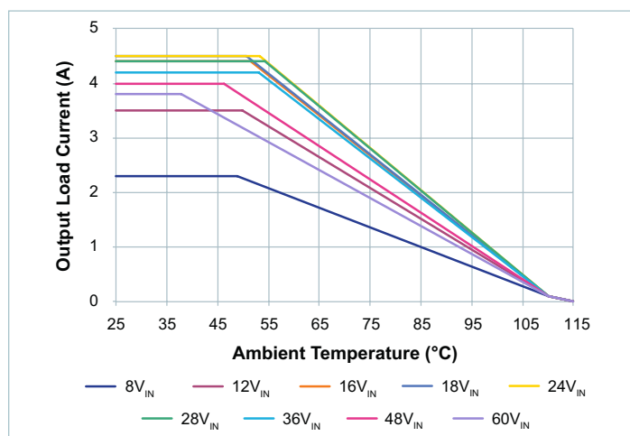
Figure 55 — Thermal de-rating PI3740-00 evaluation board at V_{OUT} = 28V , 0LFM
