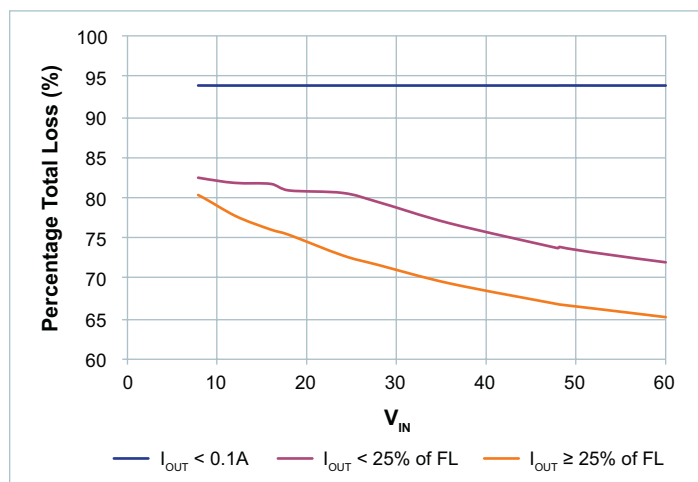
Figure 45 — V_{OUT} = 12V
