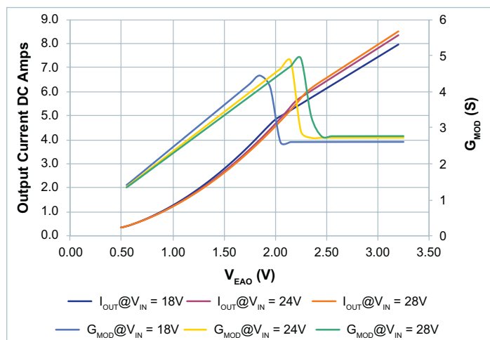
Figure 64 — G_{MOD} vs output current vs. V_{EAO} , V_{OUT} = 10V ; 18 – 28 V_{IN}
