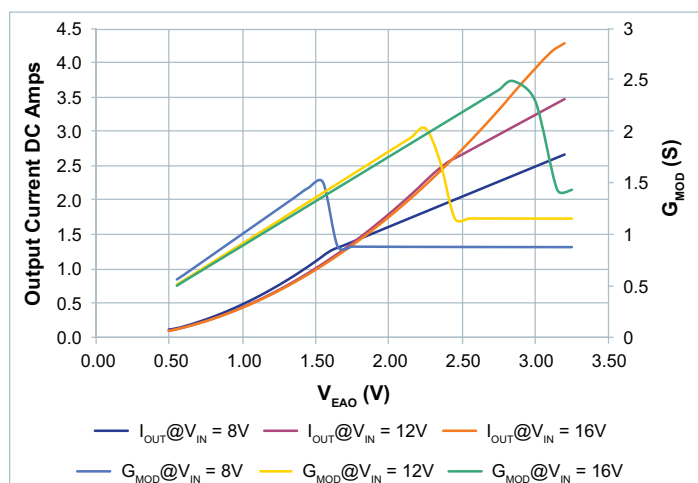
Figure 93 — G_{MOD} vs output current vs. V_{EAO} , V_{OUT} = 36V ; 8 – 16 V_{IN}
