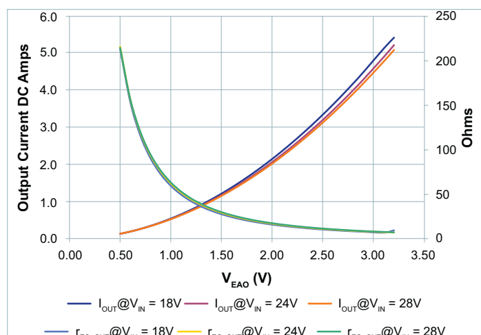
Figure 91 — r_{EQ\_OUT} vs. output current vs. V_{EAO} , V_{OUT} = 28\text{V} ; 18 – 28 V_{IN}
