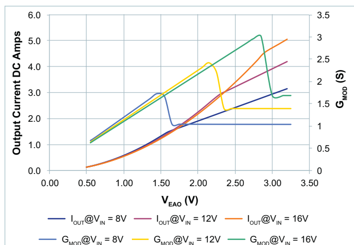
Figure 87 — G_{MOD} vs output current vs. V_{EAO} , V_{OUT} = 28\text{V} ; 8 – 16 V_{IN}
