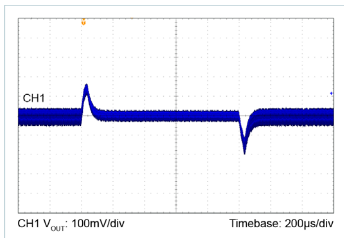
Figure 25 — 24V_{IN} to 12V_{OUT} , C_{OUT} = 8 \times 10\mu\text{F} ceramic 3.38 – 6.75A load step, 0.1A/ \mu s
