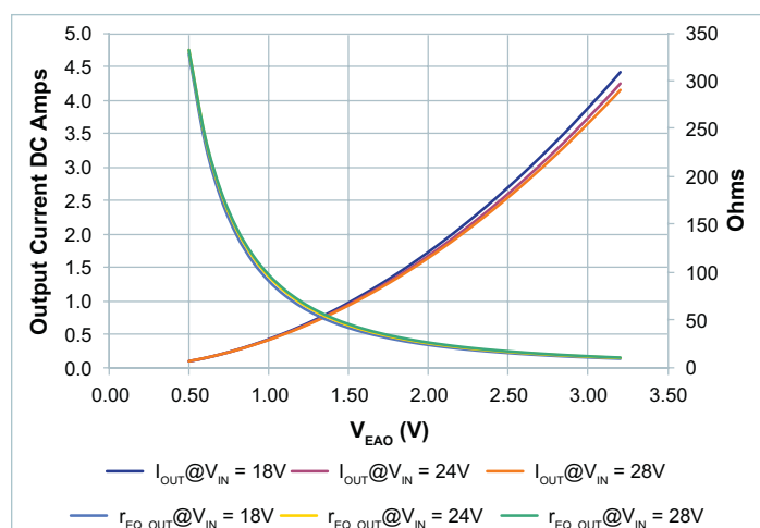
Figure 97 — r_{EQ\_OUT} vs. output current vs. V_{EAO} , V_{OUT} = 36V ; 18 – 28 V_{IN}
