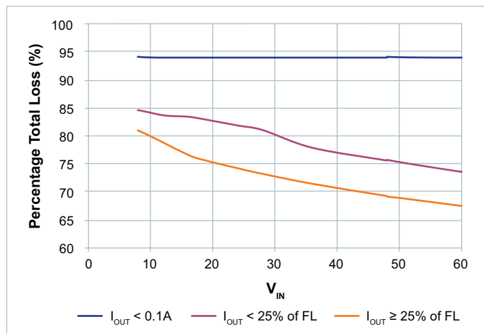
Figure 44 — V_{OUT} = 10V
