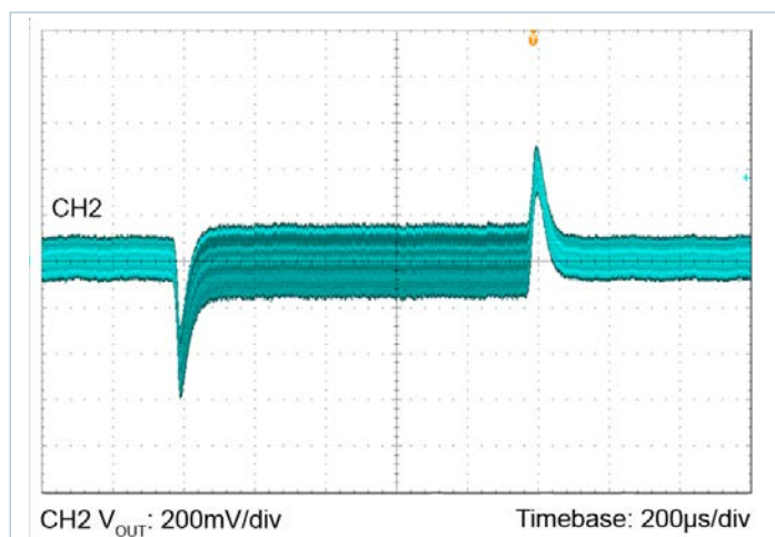
Figure 29 — 24V_{IN} to 50V_{OUT} , C_{OUT} = 8 \times 2.2\mu\text{F} ceramic 2.5 – 1.25A load step, 0.1A/ \mu s
