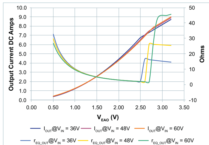
Figure 68 — r_{EQ\_OUT} vs. output current vs. V_{EAO} , V_{OUT} = 10V ; 36 – 60 V_{IN}
