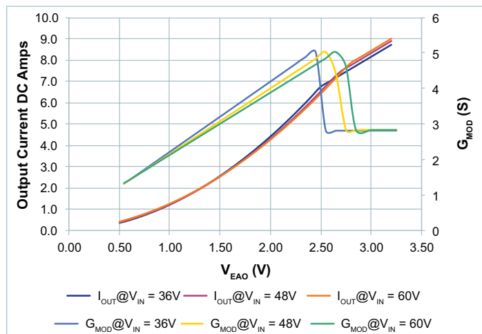
Figure 65 — G_{MOD} vs output current vs. V_{EAO} , V_{OUT} = 10V ; 36 – 60 V_{IN}
