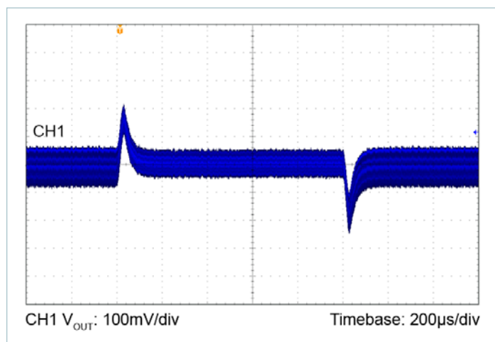
Figure 26 — 24V_{IN} to 24V_{OUT} , C_{OUT} = 8 \times 10\mu\text{F} ceramic 2.5 – 5.0A load step, 0.1A/ \mu s
