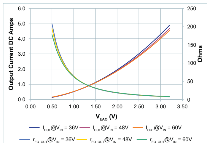
Figure 92 — r_{EQ\_OUT} vs. output current vs. V_{EAO} , V_{OUT} = 28\text{V} ; 36 – 60 V_{IN}
