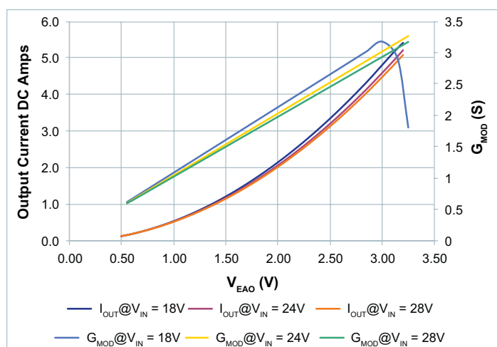
Figure 88 — G_{MOD} vs output current vs. V_{EAO} , V_{OUT} = 28\text{V} ; 18 – 28 V_{IN}
