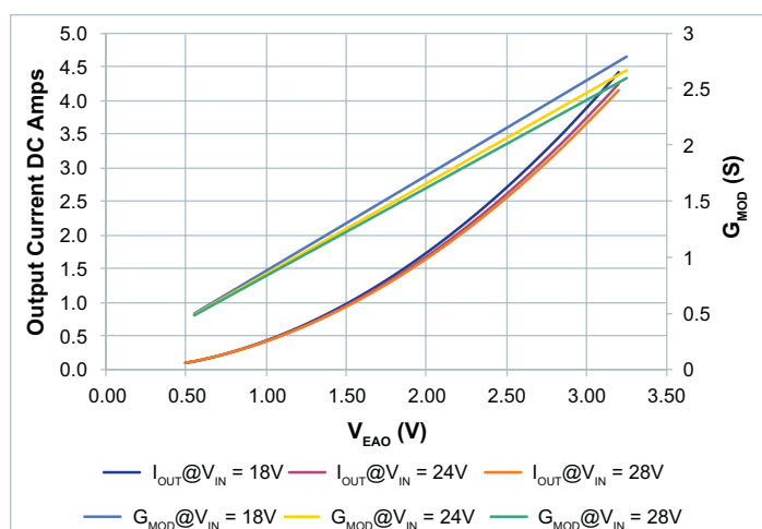
Figure 94 — G_{MOD} vs output current vs. V_{EAO} , V_{OUT} = 36V ; 18 – 28 V_{IN}
