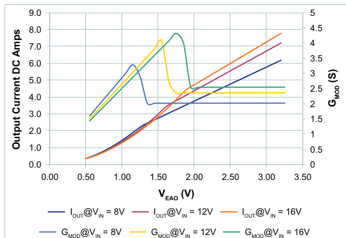
Figure 63 — G_{MOD} vs output current vs. V_{EAO} , V_{OUT} = 10V ; 8 – 16 V_{IN}
