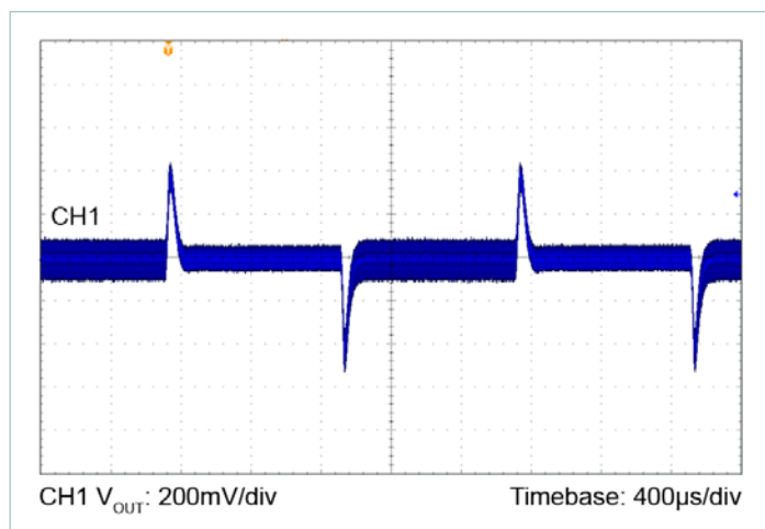
Figure 28 — 24V_{IN} to 36V_{OUT} , C_{OUT} = 8 \times 10\mu\text{F} ceramic 1.5 – 3.0A load step, 0.1A/ \mu s
