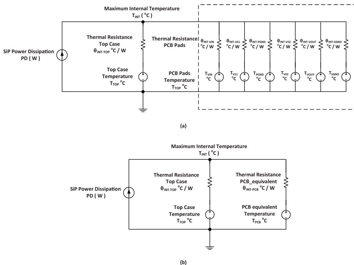
Figure 42 — PI3740-00 SiP thermal model (a) and its simplified version (b).
