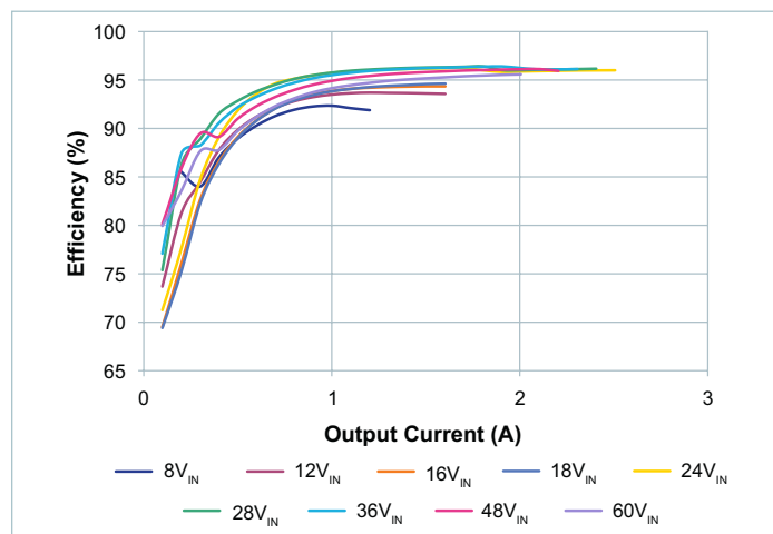
Figure 9 — 50V OUT efficiency
