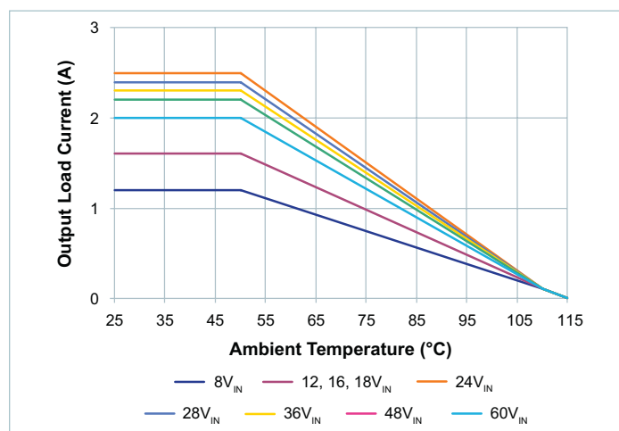
Figure 57 — Thermal de-rating for PI3740-00 evaluation board at V_{OUT} = 50V , 0LFM
