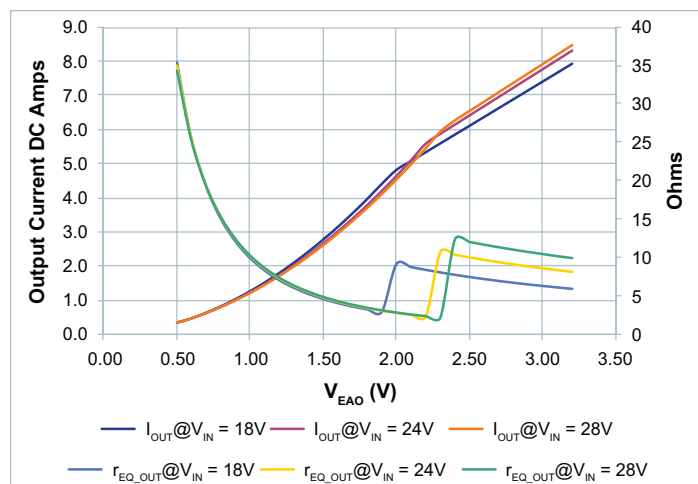
Figure 67 — r_{EQ\_OUT} vs. Output Current vs. V_{EAO} , V_{OUT} = 10V ; 18 – 28 V_{IN}
