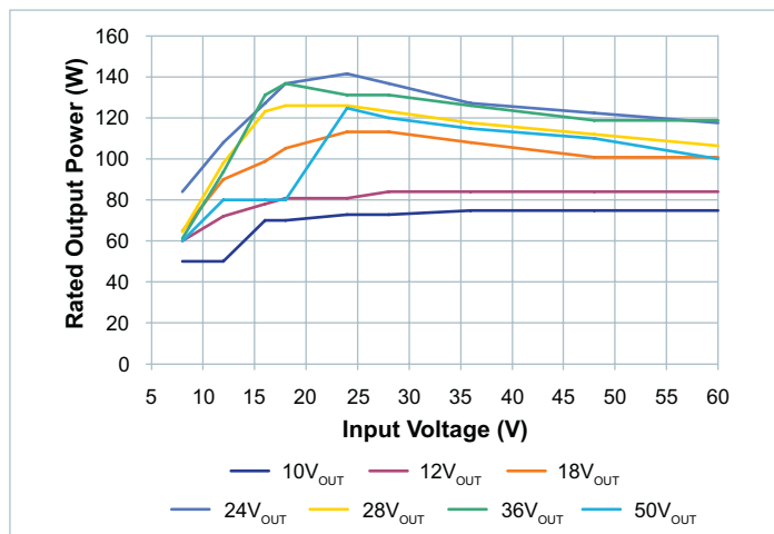
Figure 2 — Output power of PI3740-00
