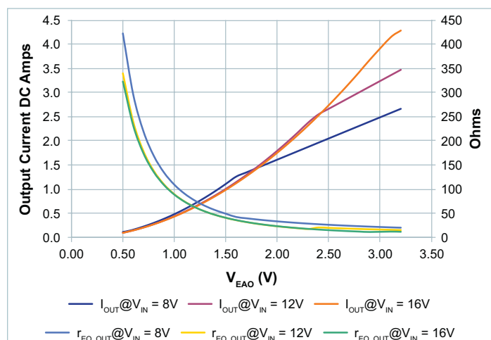
Figure 96 — r_{EQ\_OUT} vs. output current vs. V_{EAO} , V_{OUT} = 36V ; 8 – 16 V_{IN}
