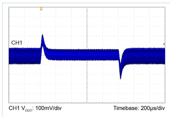
Figure 27 — 24V_{IN} to 28V_{OUT} , C_{OUT} = 8 \times 10\mu\text{F} ceramic 2.25 – 4.5A load step, 0.1A/ \mu s
