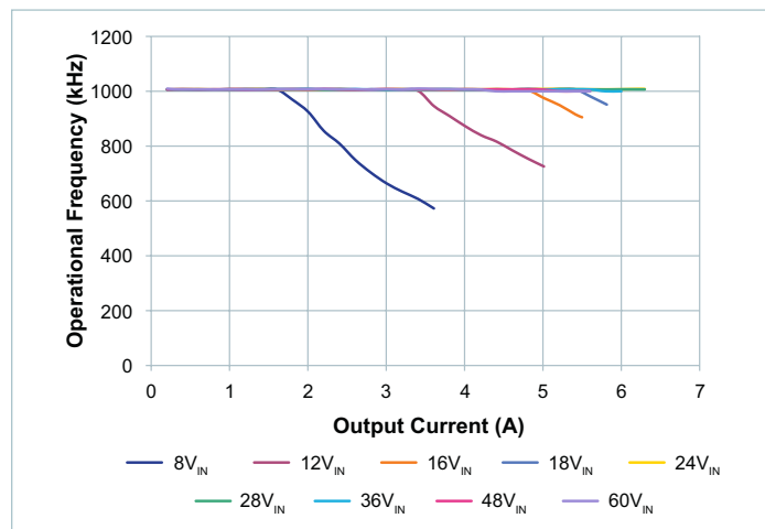
Figure 12 — Switching frequency vs. output current at 18V_{OUT}
