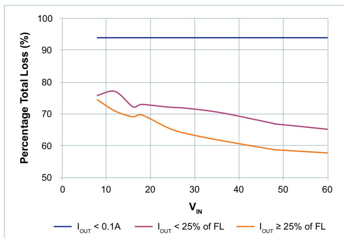
Figure 47 — V_{OUT} = 24V
