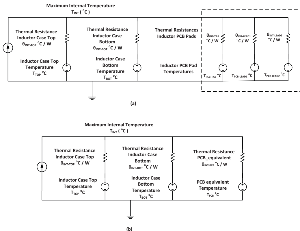
Figure 43 — PI3740-00 inductor thermal impedance model
