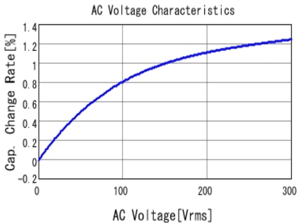
■ DE11XRA330KA4BP01F C-AC Voltage capchange, DC0V, 20.0
