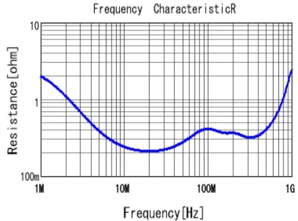
■ DE11XRA330KA4BP01F R DC0V, 20degC
