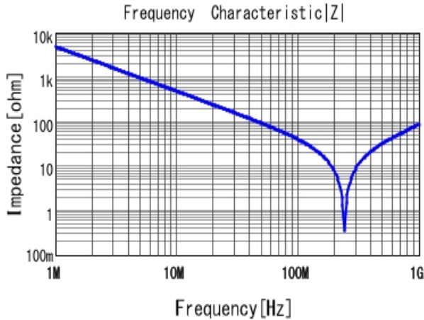
■ DE11XRA330KA4BP01F |Z| DC0V, 20degC
