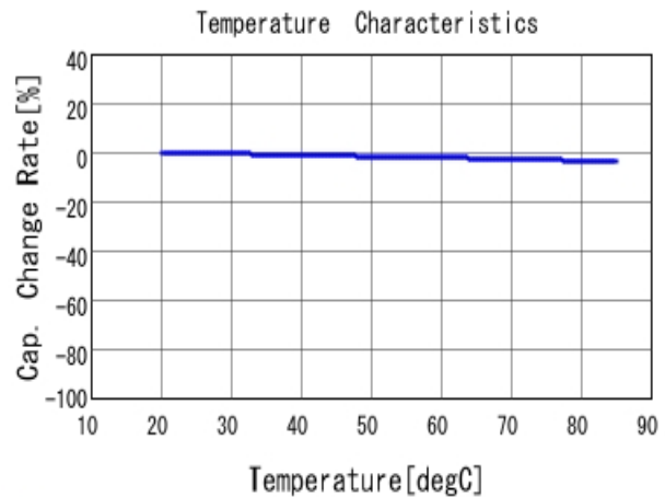
■ DE11XRA330KA4BP01F C-Temp. capchange, DC0V, AC1Vrms
