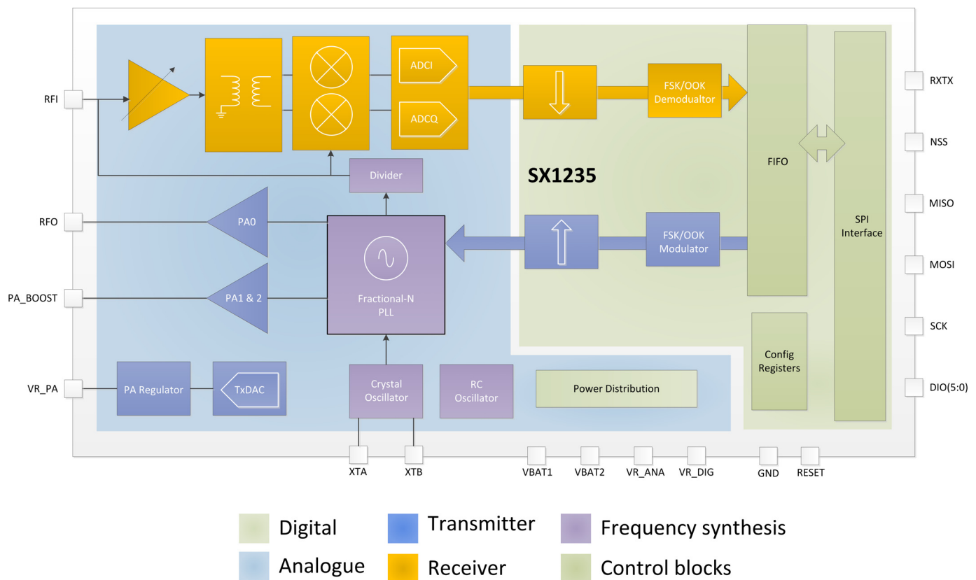
Figure 1. Block Diagram
