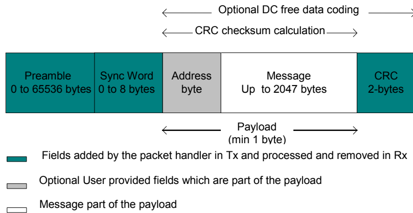
Figure 36. Fixed Length Packet Format
