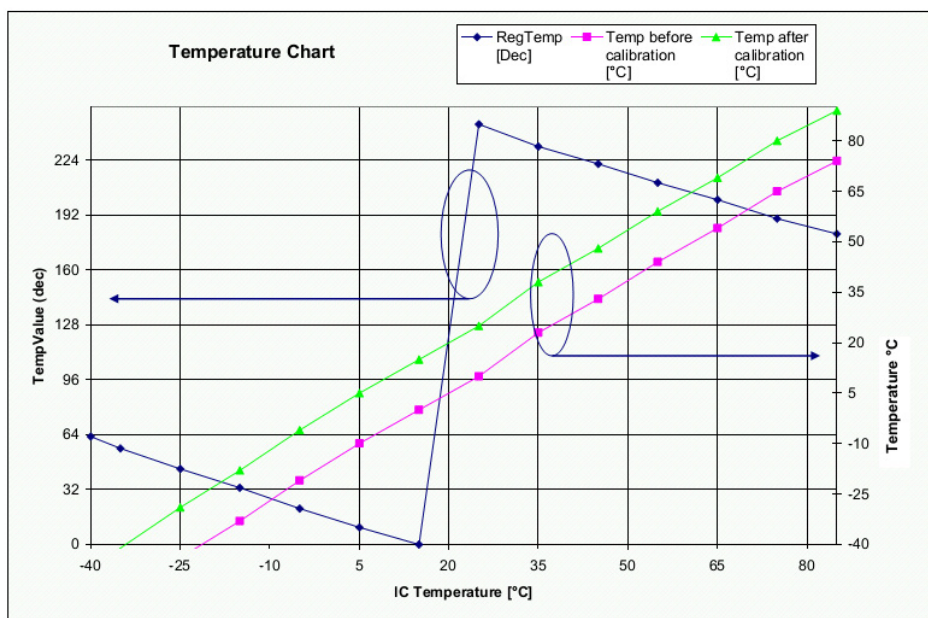
Figure 18. Temperature Sensor Response
