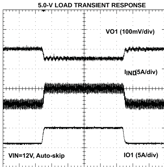
t - Time - 100 \mu s/div Figure 34.
