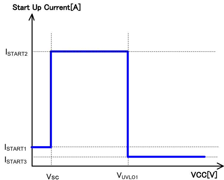
Figure 6. Start up current vs. VCC voltage
