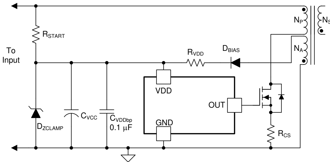
Figure 8-1. VDD Protection
