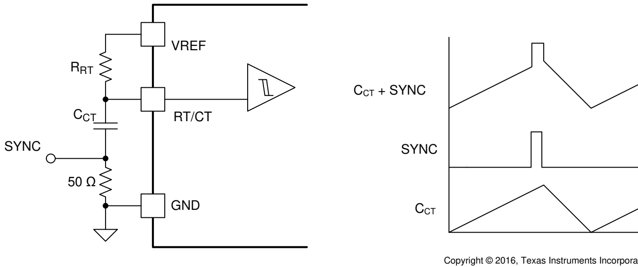
Figure 8-5. Oscillator Synchronization Circuit
