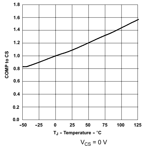
Figure 7-4. COMP to CS Offset Voltage vs Temperature V_{CS} = 0 \text{ V}
