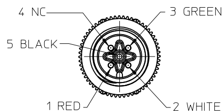
MALE INSERT - 5 POLE ENLARGED FRONT VIEW
