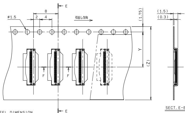
REEL DIMENSION
