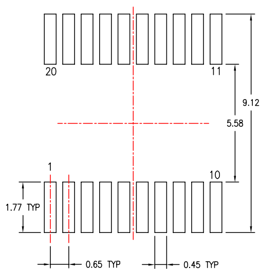
LAND PATTERN RECOMMENDATIONS
