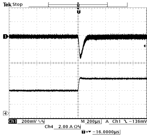
50%-75% Load Transients at V_{in}=24\text{ V}
