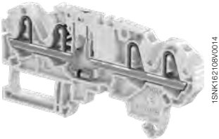
ZK2.5-CH-4P
