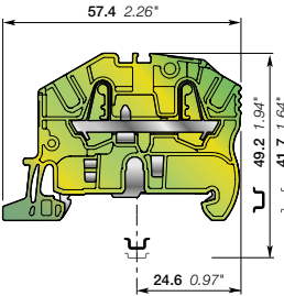
5.2 mm 0.205 in spacing
