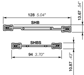
SHBS/SHB
