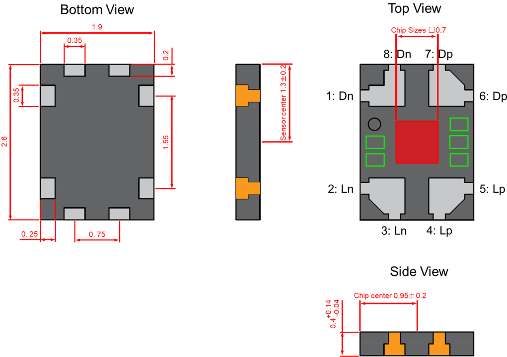
Figure 11.1 Outline Dimensions
