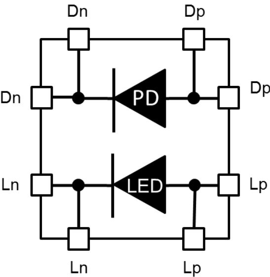
Figure 5.1 Block Diagram
