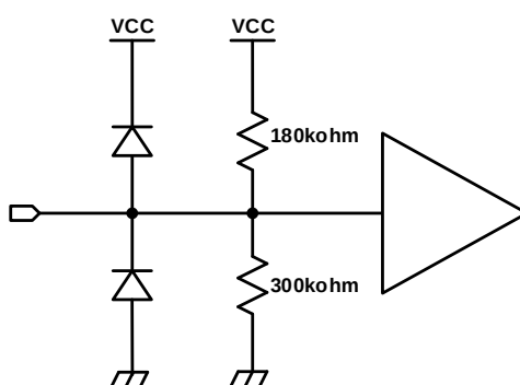
Figure 5. 4-Level LVCMOS Input Schematic Diagram
