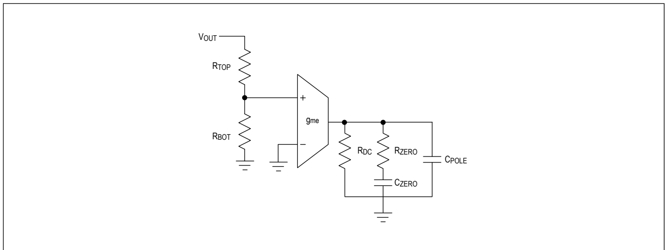
Figure 2. Setting the Output Voltage for the MAX20048
