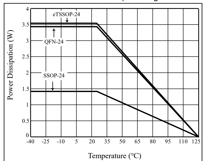
Figure 7 Dissipation Curve
