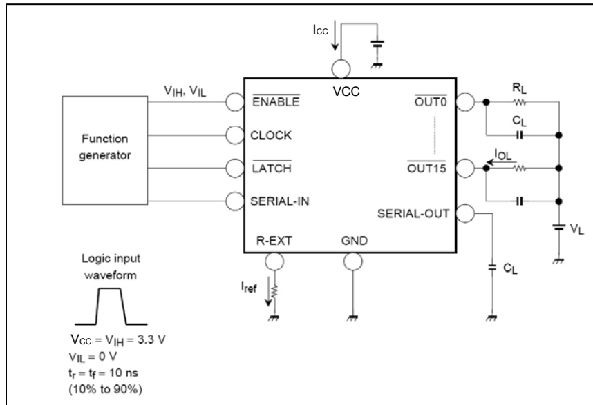
Figure 4 Test Diagram
