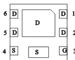
Pin Out Bottom View
