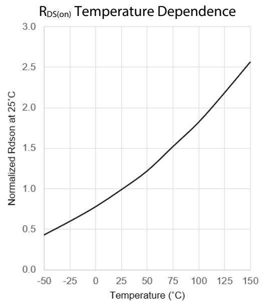
Figure 12: Normalized R_{DS(on)} as a function of T_J
