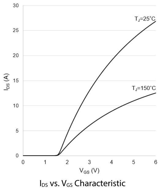
Figure 11: Typical I_{DS} vs. V_{GS}
