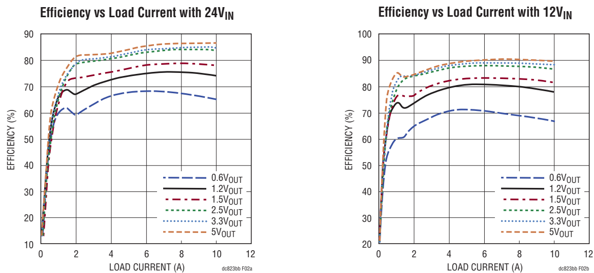
Figure 2. Measured Supply Efficiencies with Different V IN and V OUT
