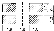
Recommended Soldering Pattern
