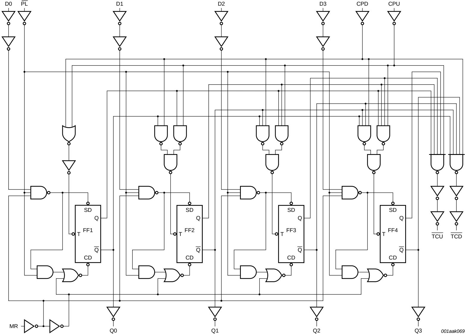
Fig 2. Logic diagram
