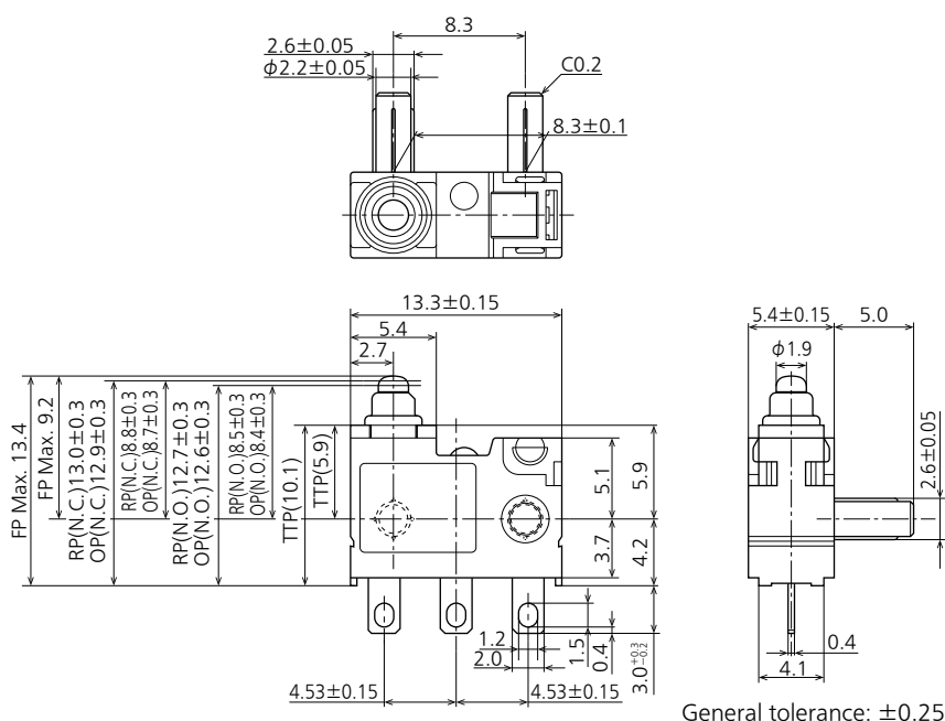
External dimensions
