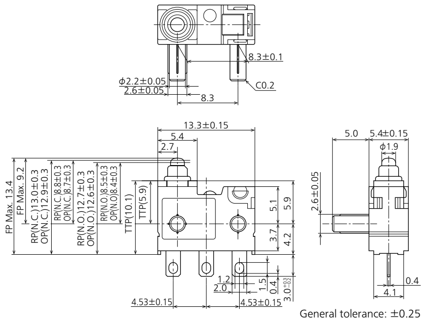
External dimensions
