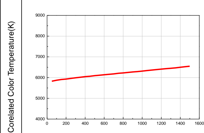
CCT vs. Forward Current ( T_{\text{soldering pad}}=25^{\circ}\text{C} )
