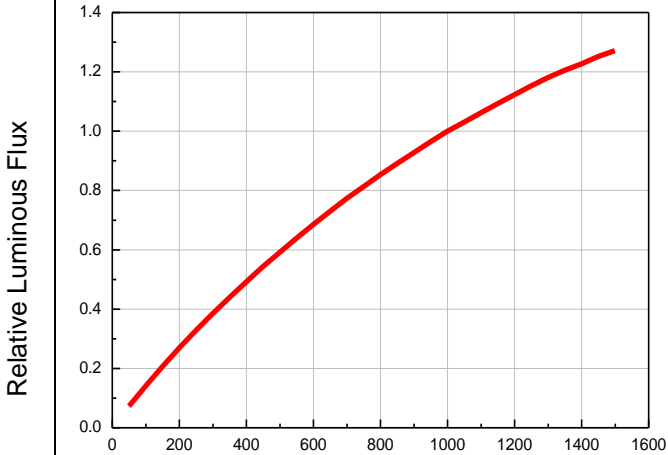
Relative Luminous Flux vs. Forward Current ( T_{\text{solder pad}}=25^{\circ}\text{C} )
