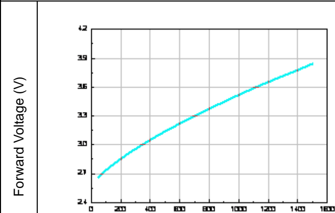
Forward Voltage vs. Forward Current ( T_{\text{solder pad}}=25^{\circ}\text{C} )
