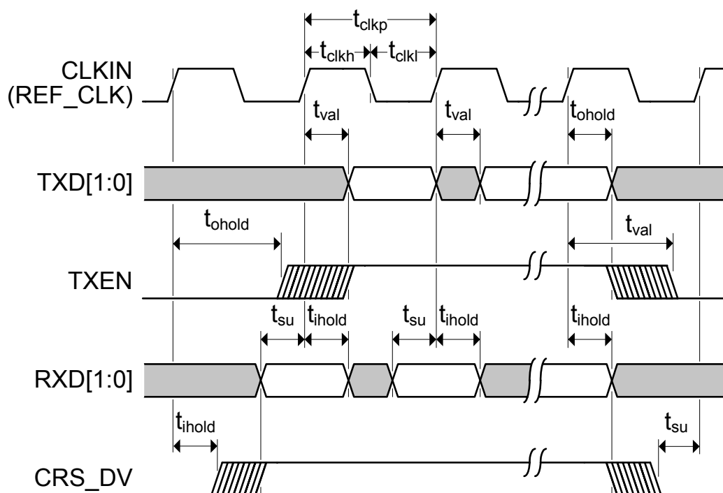
Figure 5.6 RMII Timing
