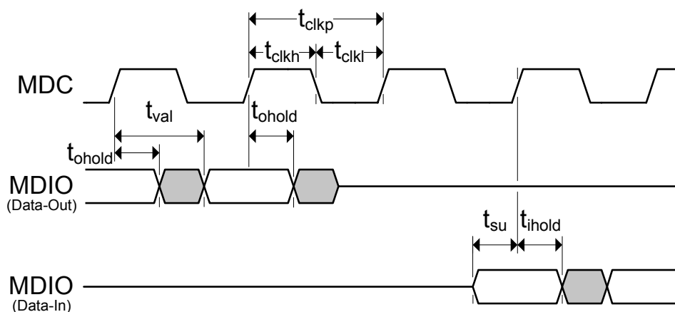
Figure 5.7 SMI Timing
