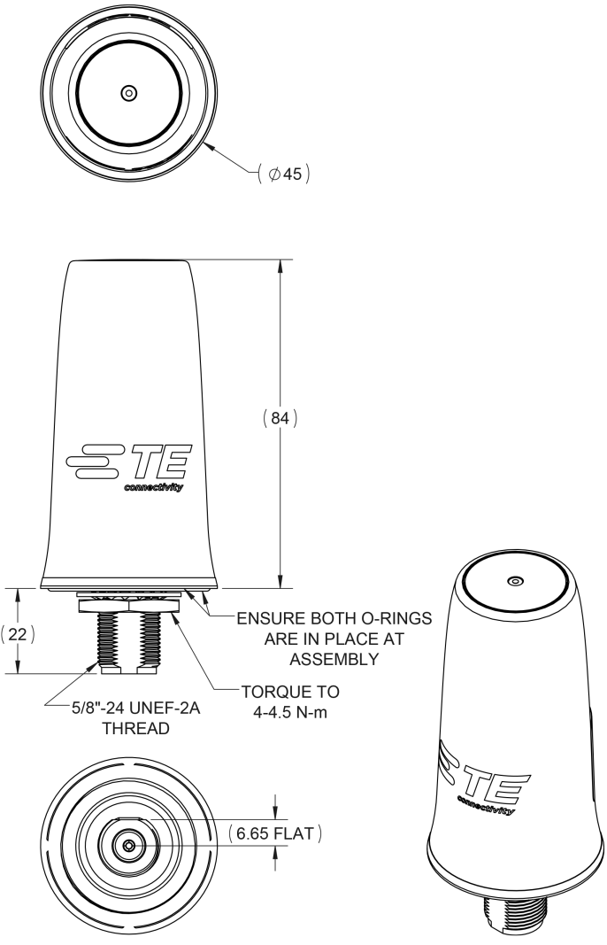
Figure 2: FTRA6971M5Px mechanical drawing
