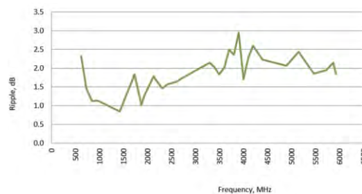
FTRA6971M5Px
