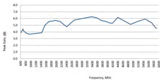
FTRA6171M5Px
