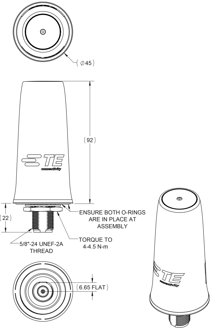
Figure 1: FTRA6171M5Px mechanical drawing
