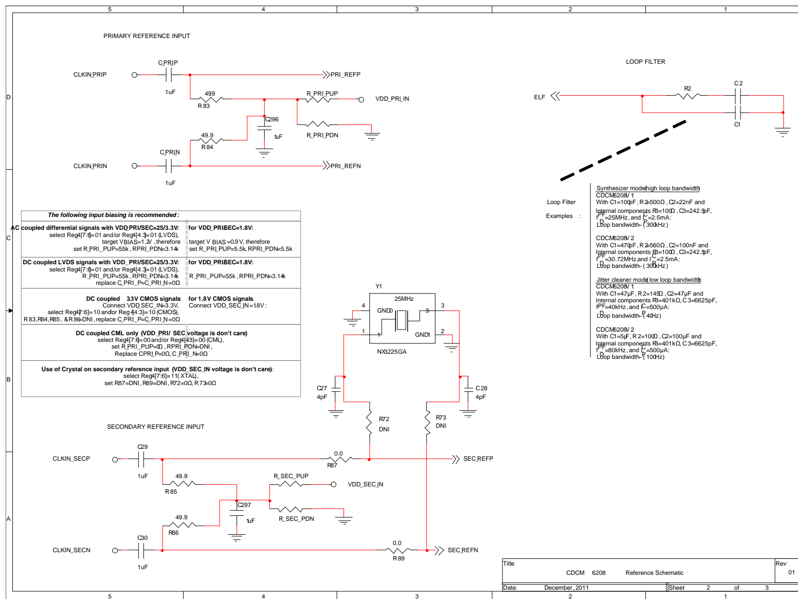
Figure 67. Schematic Page 2
