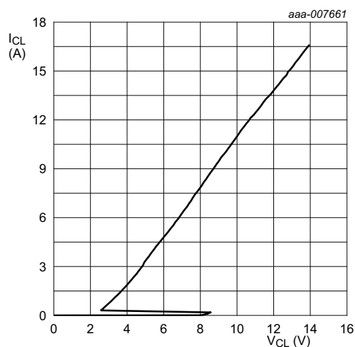
Fig 1. Dynamic resistance with positive clamping; typical values
