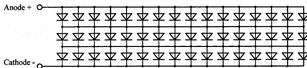
Equivalent circuit
