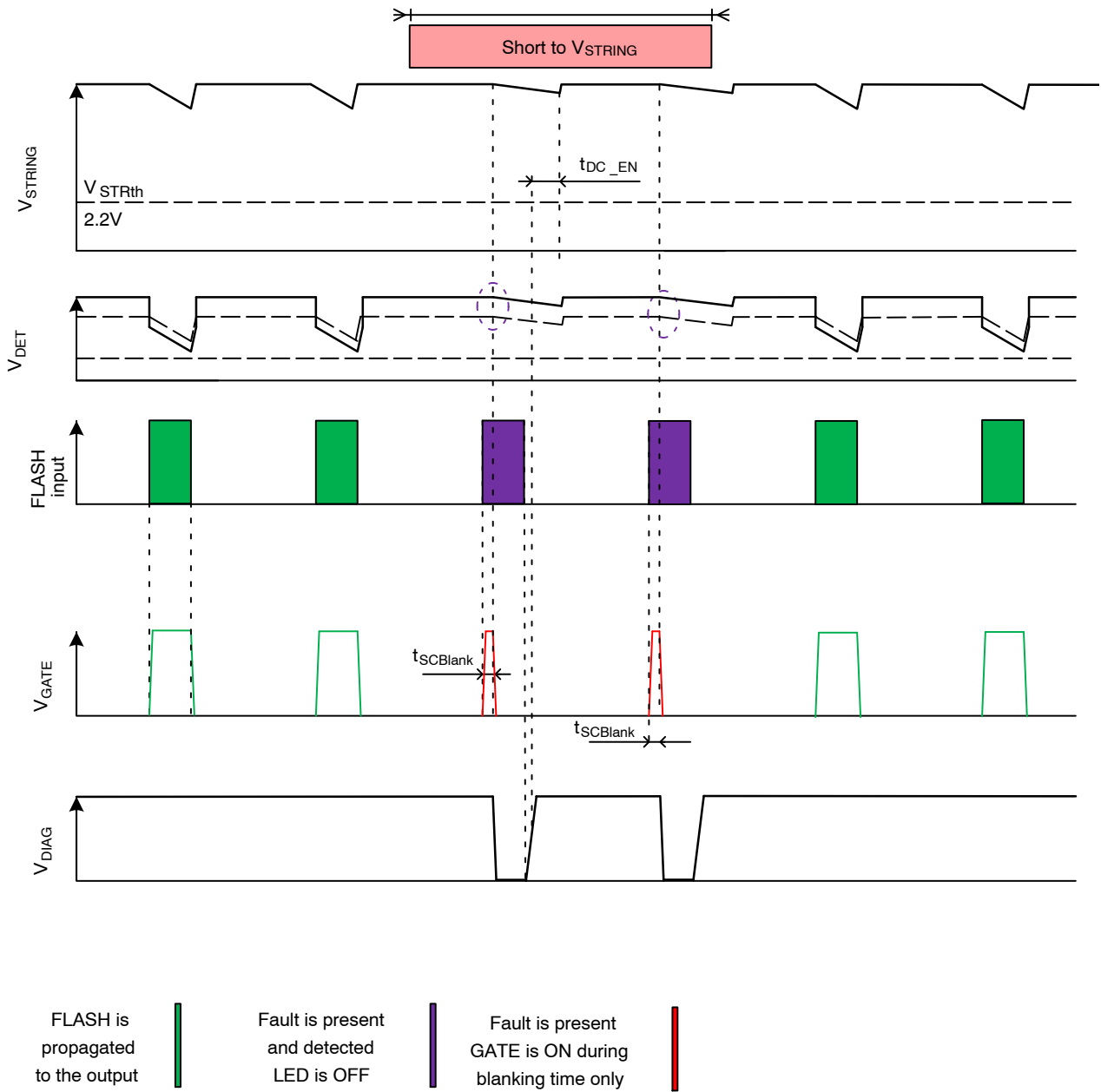
Figure 10. Timing of the Short to V_{STRING} Behavior
