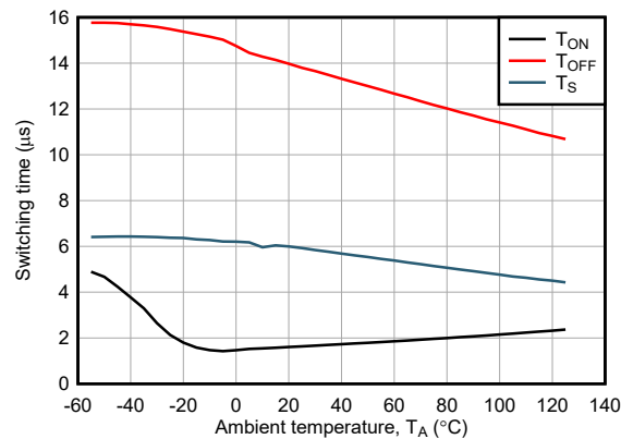
Figure 6-27. Switching Time vs Ambient Temperature
