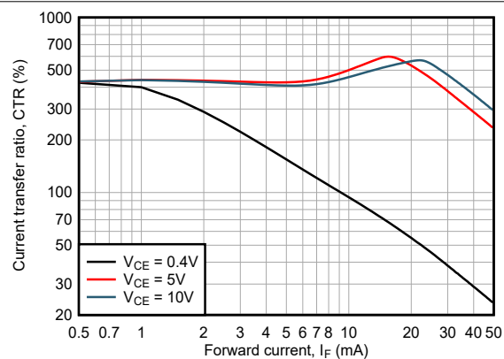
ISOM8113 & ISOM8118 T_A = 25^\circ\text{C}
