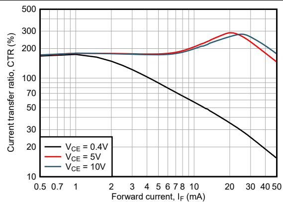
ISOM8111 & ISOM8116 T_A = 25^\circ\text{C}
