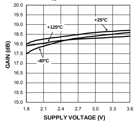
Gain vs Supply Voltage f_{RF} = 433.92\text{MHz}
