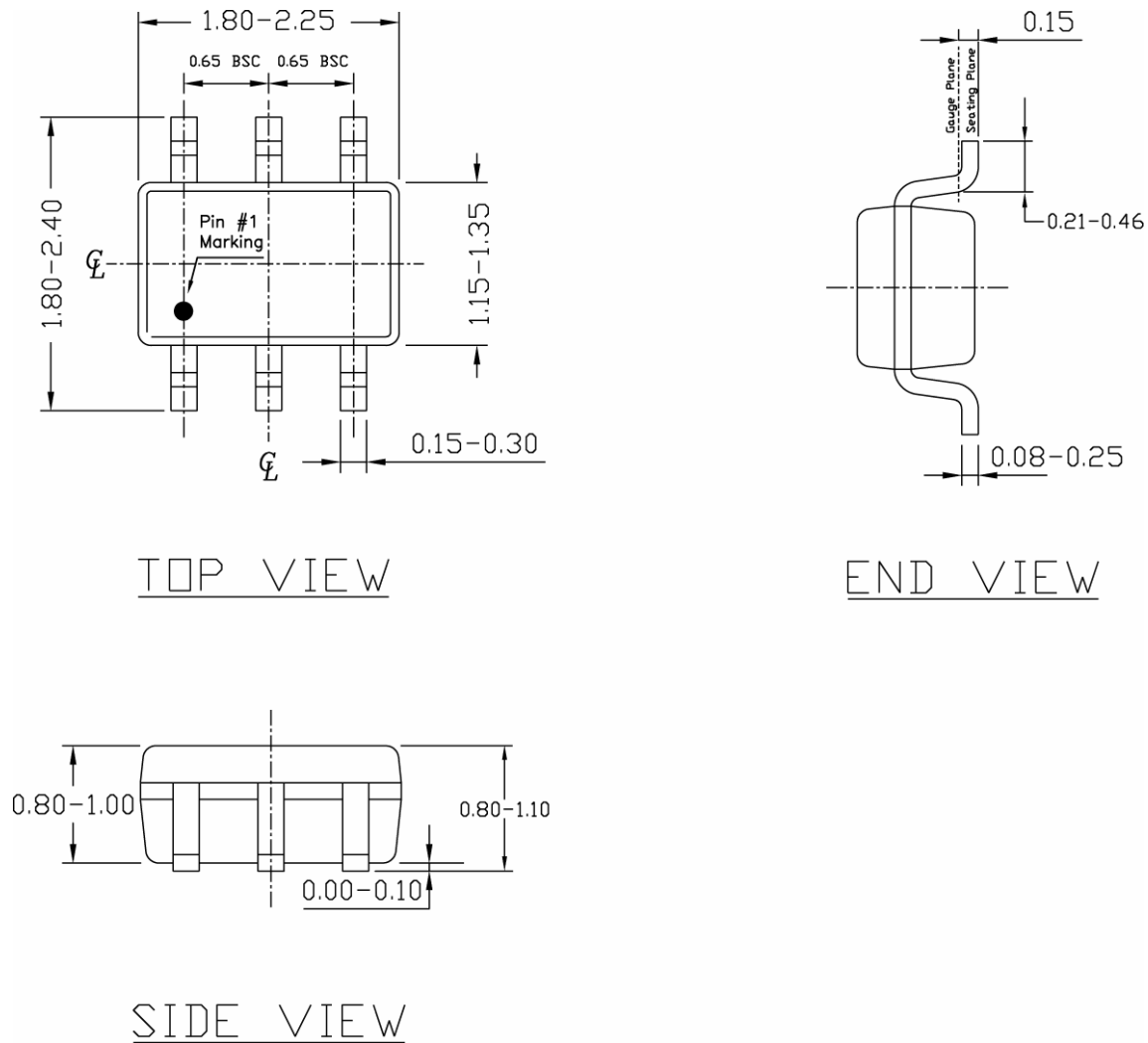
SC70-6 (C6)
