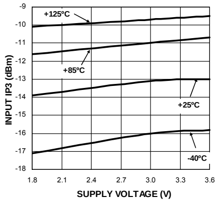
IIP3 vs Supply Voltage f_{RF} = 433.92\text{MHz}
