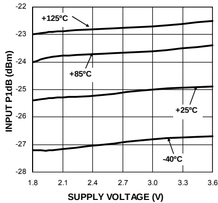
Input P1dB vs Supply Voltage f_{RF} = 433.92\text{MHz}
