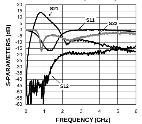
S-Parameters vs Frequency f_{RF} = 900\text{MHz} (matched)
