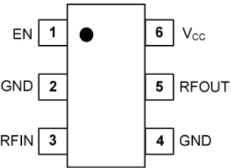
SC70-6 (C6)
