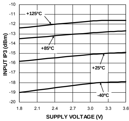
IIP3 vs Supply Voltage f_{RF} = 315\text{MHz}
