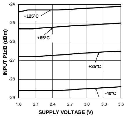
Input P1dB vs Supply Voltage f_{RF} = 315\text{MHz}
