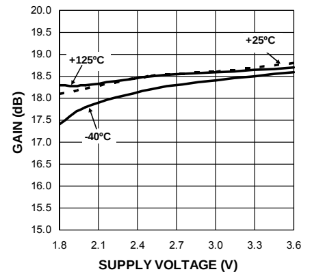
Gain vs Supply Voltage f_{RF} = 315\text{MHz}
