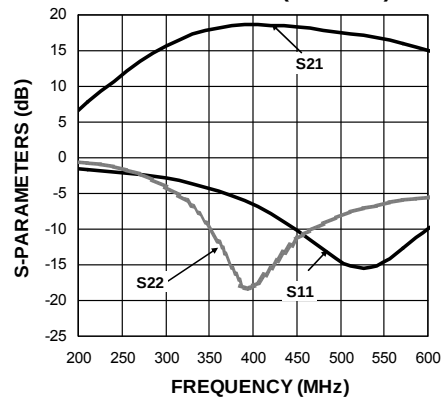
S-Parameters vs Frequency f_{RF} = 433.92\text{MHz} (matched)
