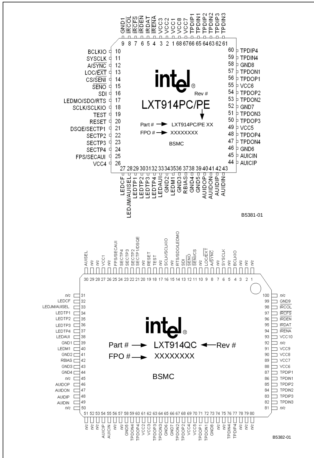
Figure 2. Pin Assignments
