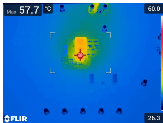
LT80603 EVALUATION BOARD CONDITIONS: 5V OUTPUT, 3.5A, f_{SW} = 400\text{kHz}
