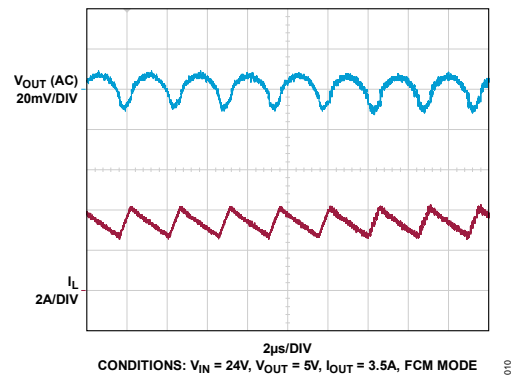
Figure 10. Steady State Switching Waveform
