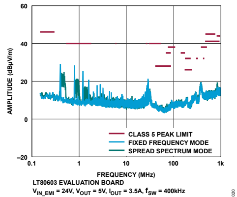
Figure 20. CISPR25 Radiated Emission Test with Class 5 Peak Limits
