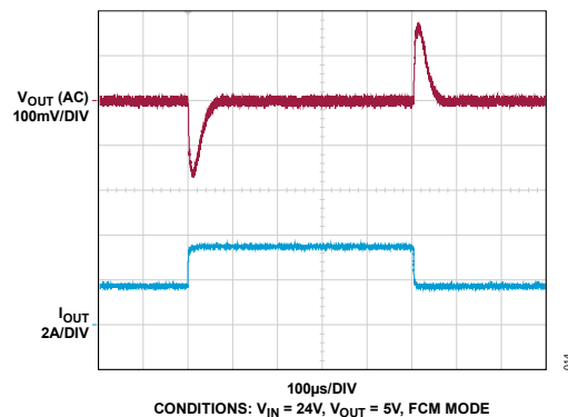
Figure 14. Load Current Stepped from 1.75A to 3.5A
