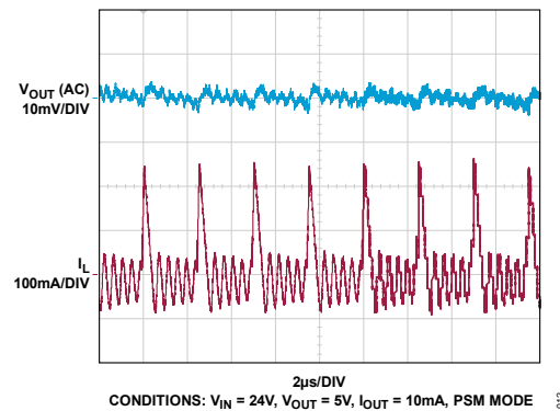
Figure 12. Steady State Switching Waveform
