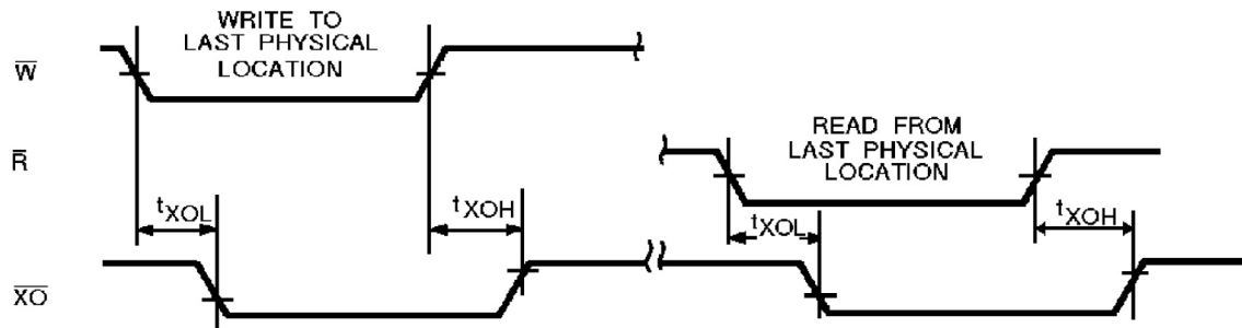
Figure 16. Expansion Out
