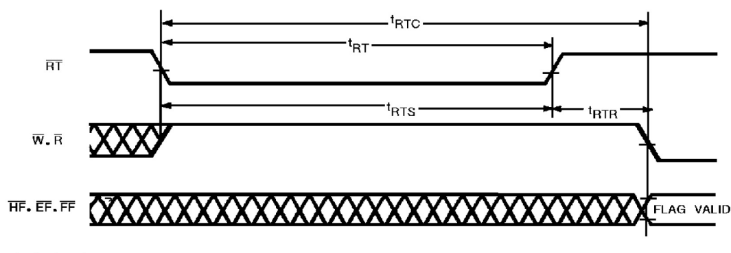
Figure 12. Retransmit
