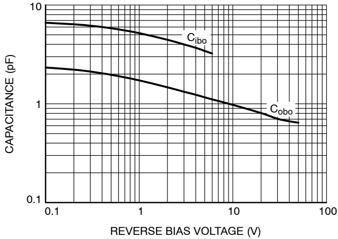
Figure 16. Capacitance
