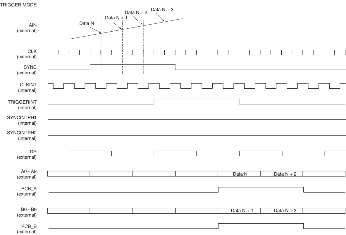
Figure 4-2. Trigger Mode Diagram
