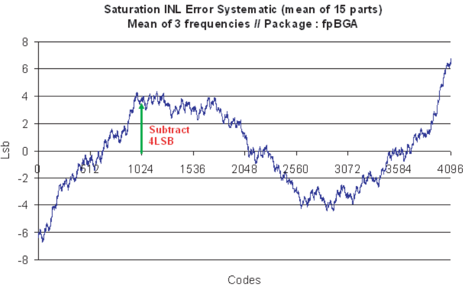
Figure 6-7. INL Calibration
