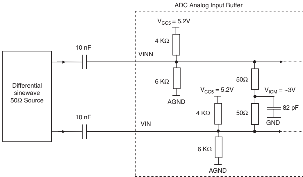
Figure 6-3. Differential Analogue Input Implementation (AC Coupled)
