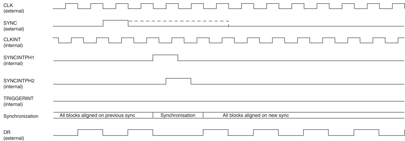
Figure 2-4. SYNC Timing Diagram (1:1 DMUX)
