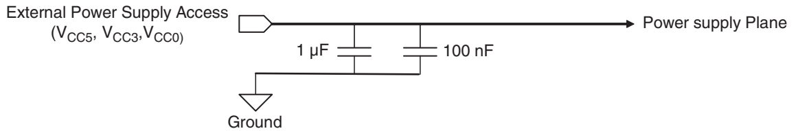
Figure 6-1. EV12AS200 Power Supplies Decoupling and Grounding Scheme
