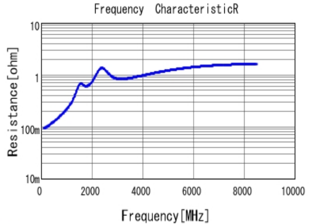
■ GRM1555C1H151GA01 R DC0V, 25degC
