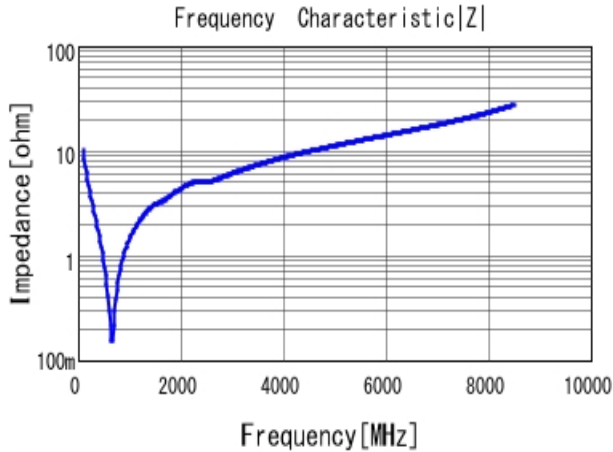
■ GRM1555C1H151GA01 |Z| DC0V, 25degC
