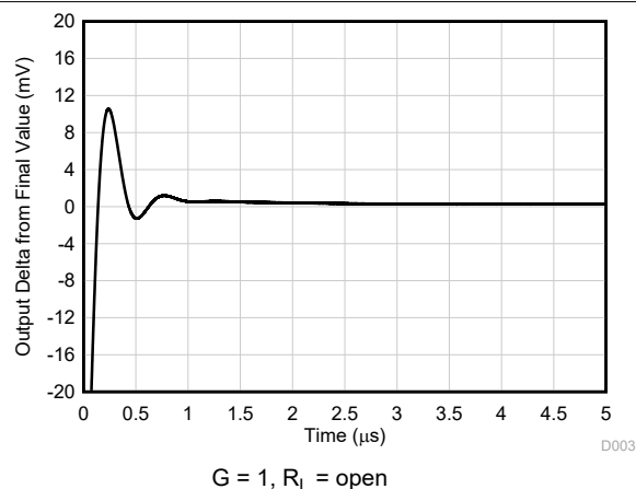
Figure 7-31. Large-Signal Step Response (Rising)
