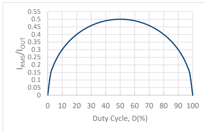
Figure 8: Normalized Input Capacitor Ripple versus Duty Cycle
