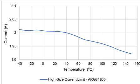
High-Side Current Limit vs. Temperature – ARG81800
