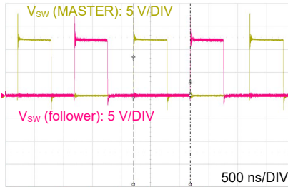
Interleaved Clock Generation V_{OUT} = 5.0\text{ V} , f_{SW} = 500\text{ kHz} , PWM Mode
