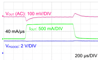
Load Transient Performance V_{OUT} = 3.3\text{ V} , PWM Mode
