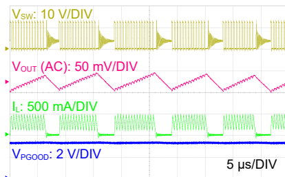
Steady-State Performance V_{OUT} = 3.3\text{ V} , I_{OUT} = 100\text{ mA} , LP Mode
