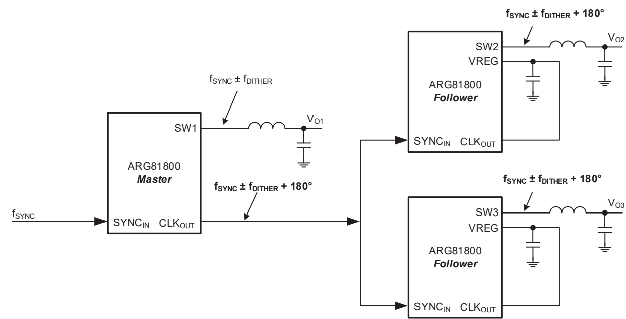
Figure 1: Master-Follower Configuration
