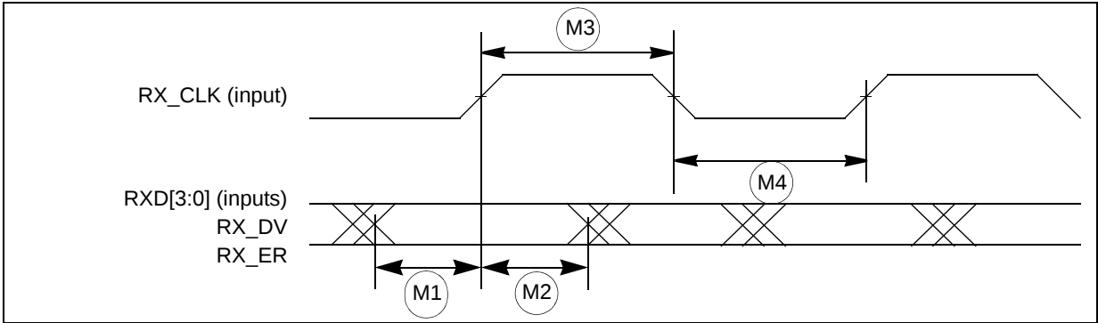
Figure 22. MII receive signal timing diagram
