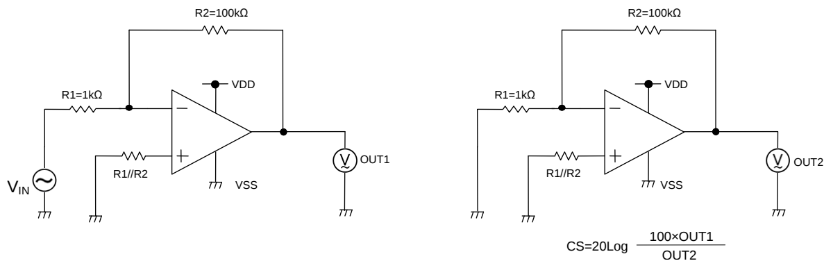
Figure 51. Test circuit 3 (Channel Separation)
