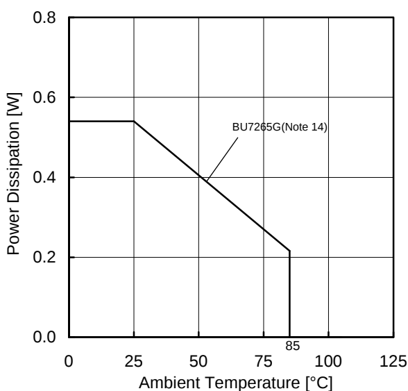
(c)BU7265G
