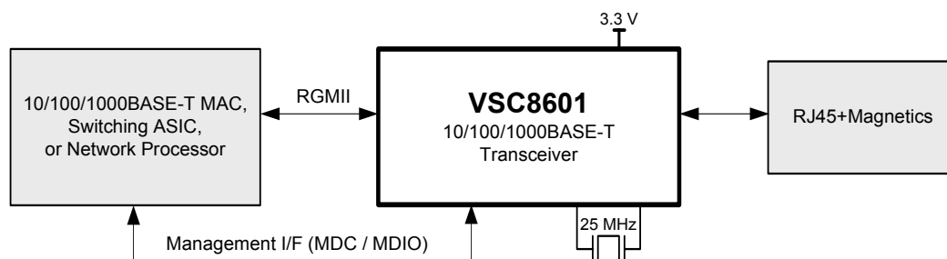
Figure 1. Typical Application
