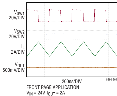
Switching Waveforms (Buck Region)
