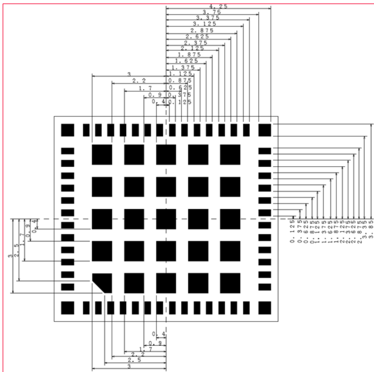
Figure 21: Land Pattern
