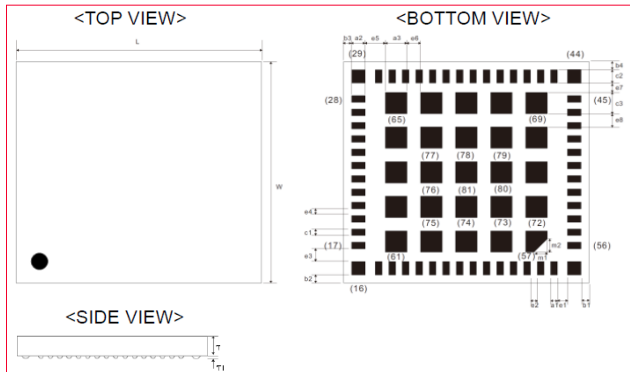
Figure 26: Product Dimension
