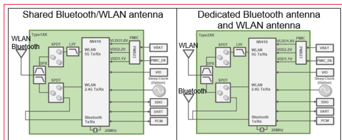
Figure 25: Shared Bluetooth/WLAN Antenna and Dedicated Bluetooth/WLAN Antenna
