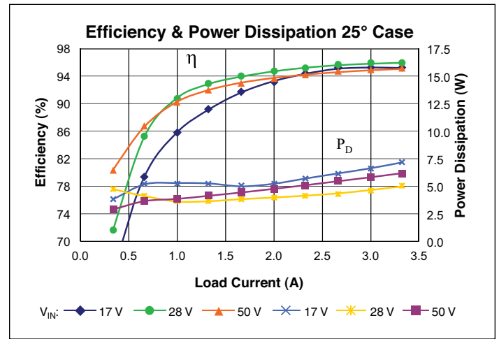
Figure 7 — Efficiency and power dissipation vs. output current at 36 V_{OUT} , 25^{\circ}\text{C} T_{CASE}
