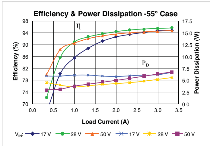
Figure 6 — Efficiency and power dissipation vs. output current at 36 V_{OUT} , -40^{\circ}\text{C} T_{CASE}
