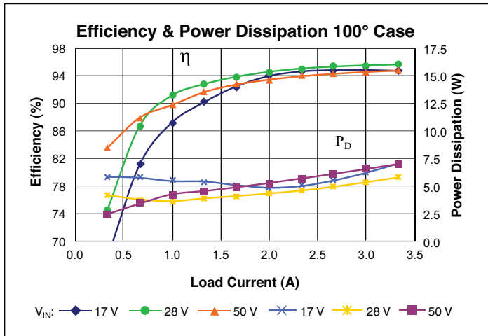
Figure 8 — Efficiency and power dissipation vs. output current at 36 V_{OUT} , 100^{\circ}\text{C} T_{CASE}
