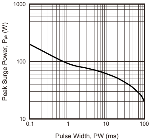
Fig.4 - Maximum Surge Power
