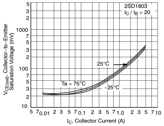
Figure 14. V_{CE(sat)} - I_C
