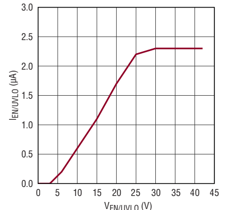
EN/UVLO Current vs Voltage
