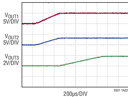
Start-Up Sequence
