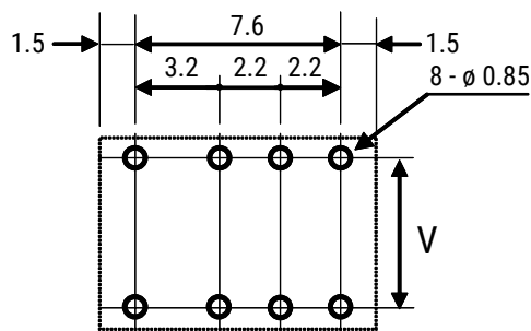
UC2 Series (bottom view)
