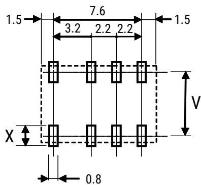
UD2 Series (top view)
