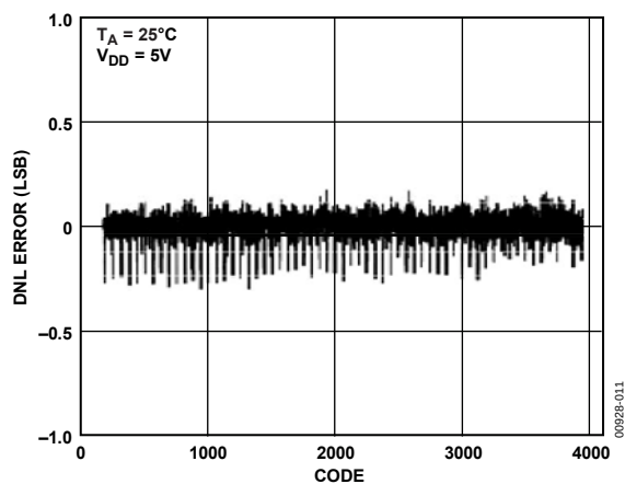
Figure 11. AD5322 Typical DNL Plot
