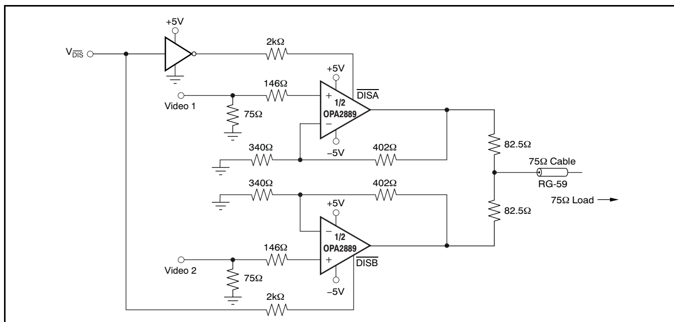
Figure 55. 2-Channel Video Multiplexer (SO-14 package only)
